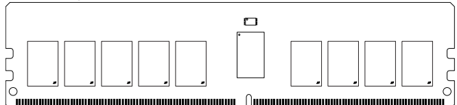
Figure 1: 288-Pin RDIMM (MO-309, R/C-C1, R/C-C2)
